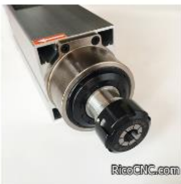
GDZ93X82-3.5 3.5kW Air Cooled CNC Spindle Motor With ER25 collet for Woodworking CNC Router
